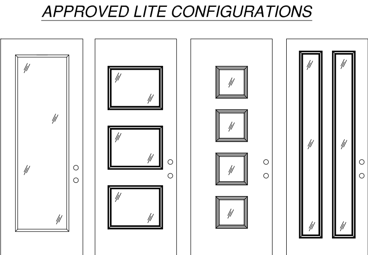
APPROVED LITE CONFIGURATIONS LITE CONFIGURATIONS SHOWN ARE FOR REFERENCE ONLY. MULTIPLE LITE CONFIGURATIONS ARE APPROVED AS LONG AS LITE SIZE DOES NOT EXCEED 11.5 FT 2
