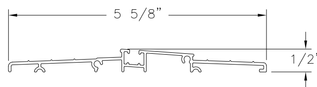
ADA THRESHOLD
