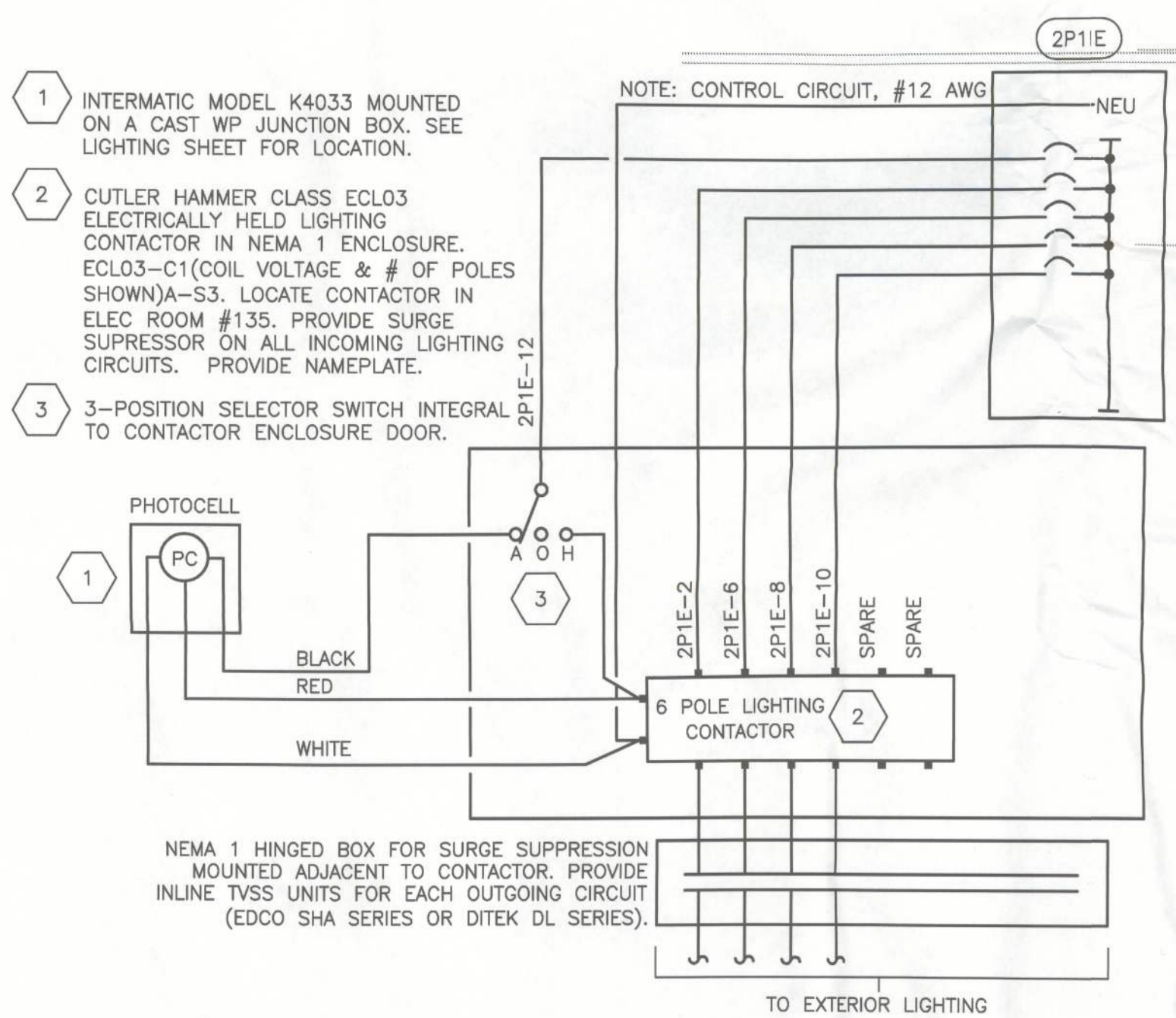
EXTERIOR LIGHTING CONTROL DIAGRAM NOT TO SCALE
