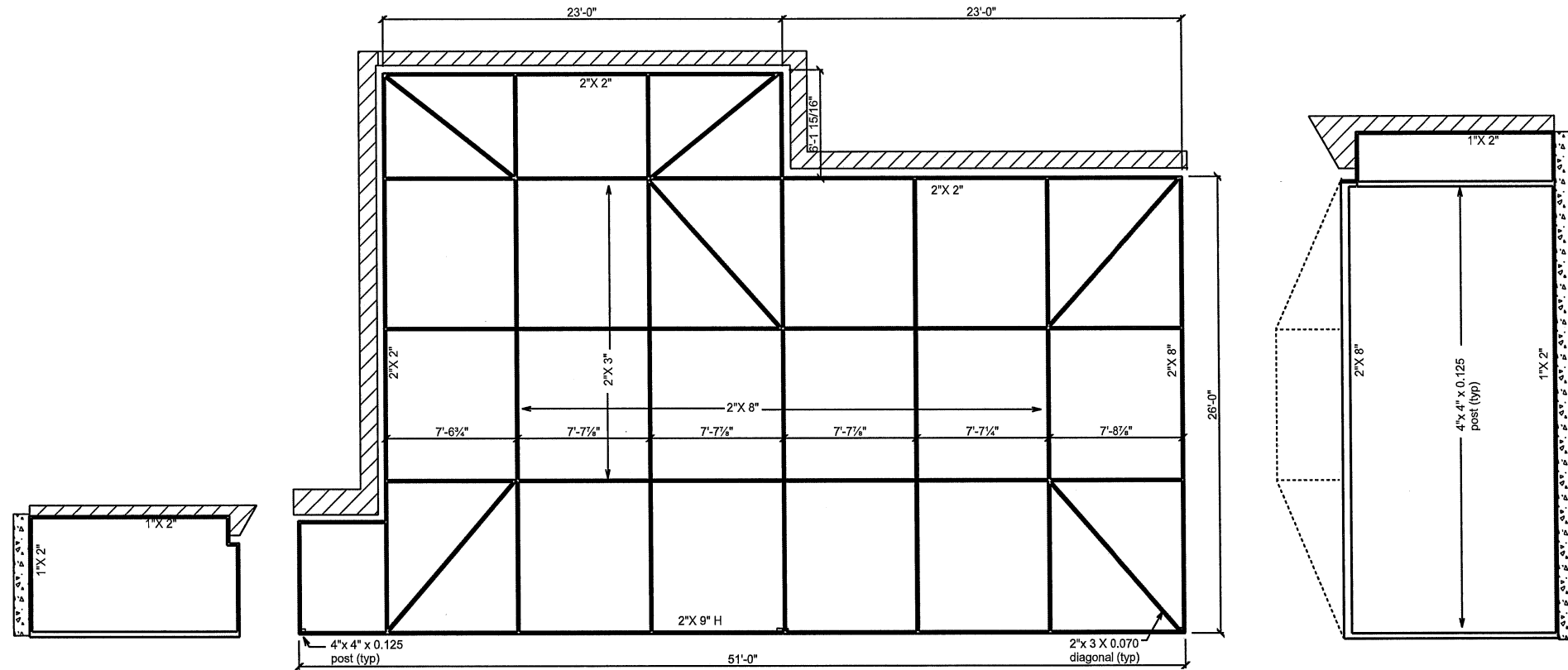
PLAN VIEW
