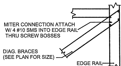
DIAGONAL ROOF BRACE DETAIL PLAN VIEW
