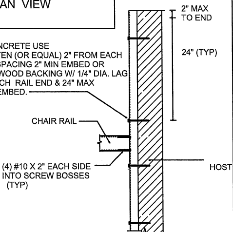
RAIL TO HOST @ CHAIR RAIL CONNECTION WOOD OR MASONRY HOST CHOOSE CONNECTOR THAT IS APPLICABLE N.T.S.
