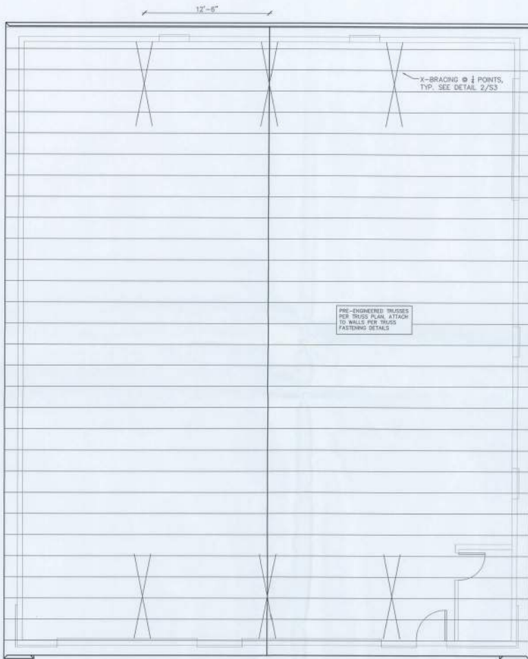
ROOF PLAN 1/4"=1'-0"
