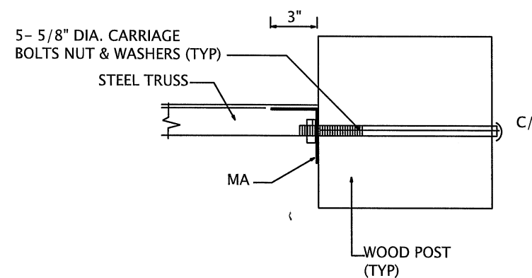
TRUSS TO POST DETAIL PLAN VIEW
