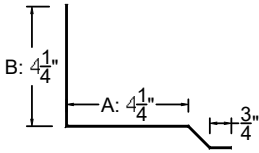
SIDEWALL (10")
