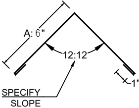
FLAT CAP (14")
