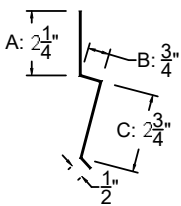
REGULAR STUCCO (6")
