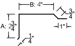
GABLE (8.75")
