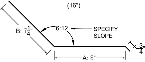
TRANSITION (16")
