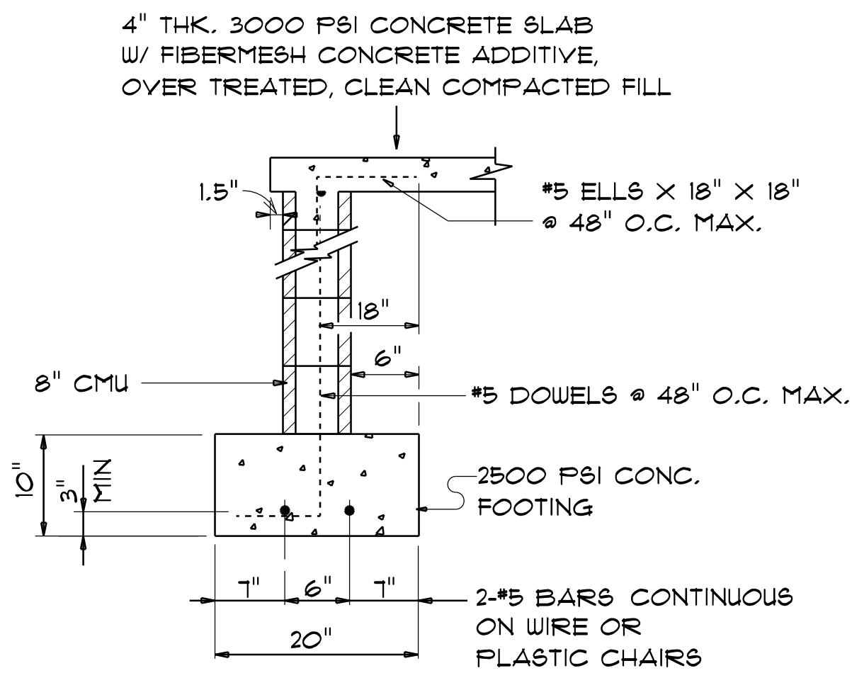
PORCH / CARPORT STEMWALL DETAIL SCALE: 3/4" = 1'-0" C S.4
