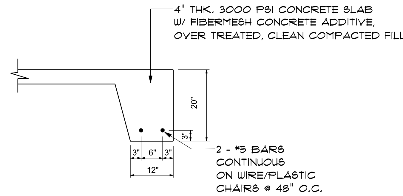
SECTION D SCALE: not to scale S.4
