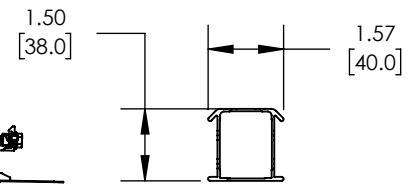
FRONT VIEW RAIL
