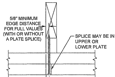
OFFSET 1/4" FROM TOP PLATE SPLICE FOR FULL VALUES
