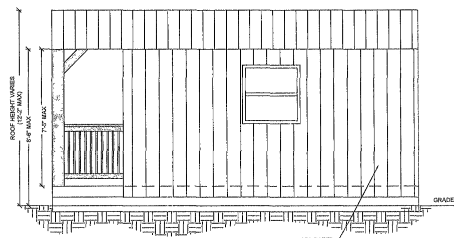
REAR ELEVATION
