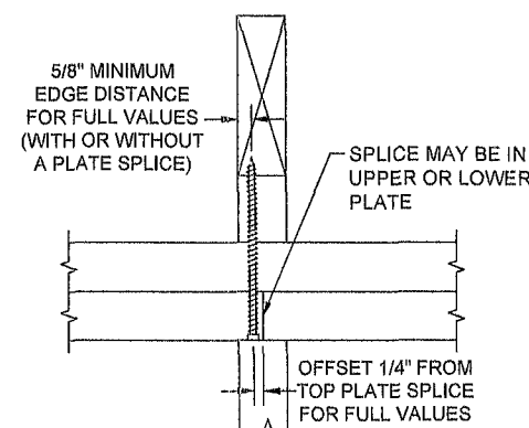
MINIMUM EDGE DISTANCE AND TOP-PLATE SPLICE OFFSET
