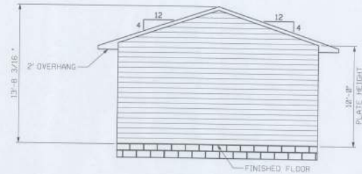
LEFT ELEVATION
