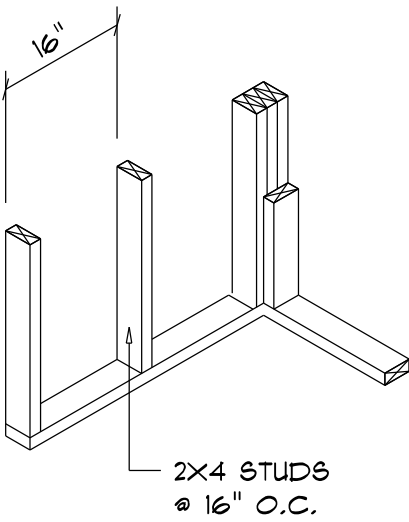
WALL CORNER
